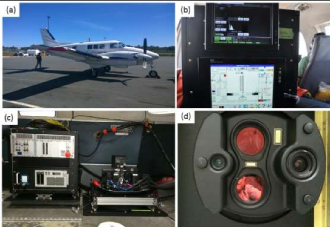
Figure 3 (a) Aircraft used for September 2014 lidar survey; (b) display monitors on a rack as seen by lidar operator in-flight; (c) main body of sensor control rack (left) and lasers and cameras located over the hole cut in the bottom of the plane (right); (d) large red circles are the lasers; the RCD30 lens (right) and low resolution camera (left) as seen from the bottom of the aircraft.
