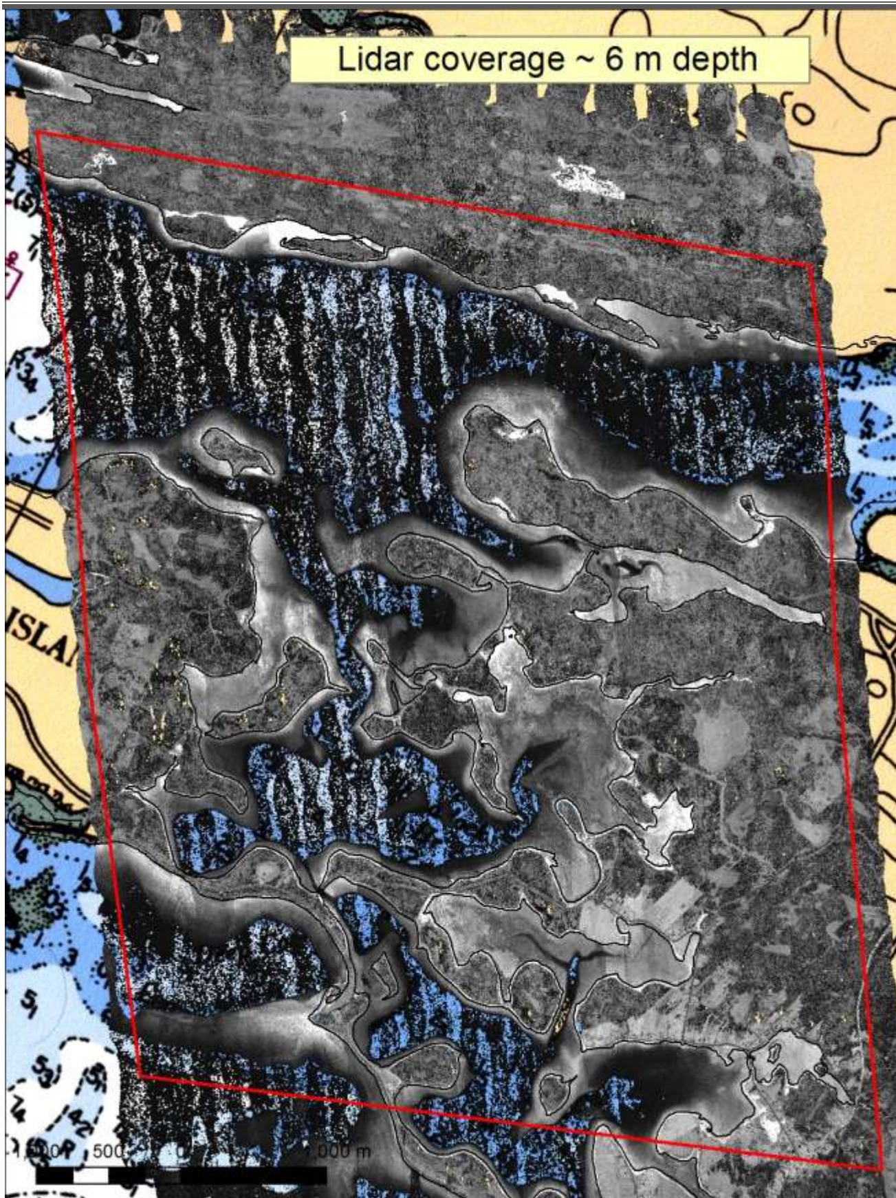
Figure 8 Example of the green laser raw reflectance image overlaid on a CHS chart of the area.
