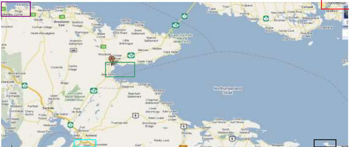
Figure 32 Location map of sites (coloured rectangles) along the Northumberland Strait. Sites of interest include Cape John (black), Charlottetown (red), Port Elgin (green), and Shediac (purple). Nappan (blue) along the upper Bay of Fundy is also on the map.
